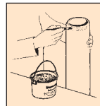
Lubrication of pipe end before joining
